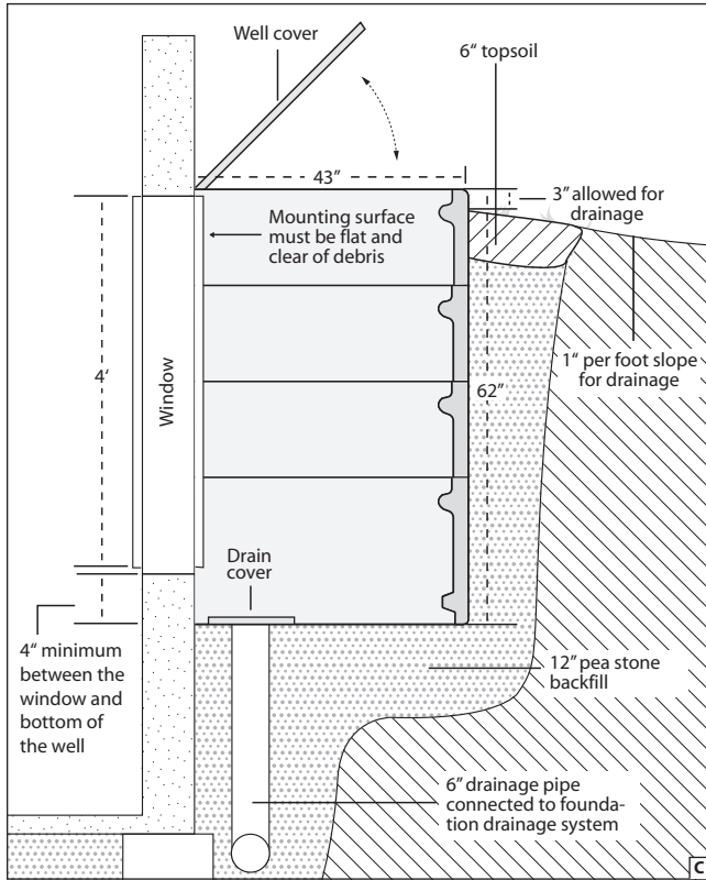
Side view of well installation
